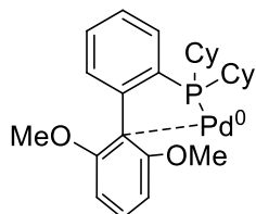
JohnPhos
